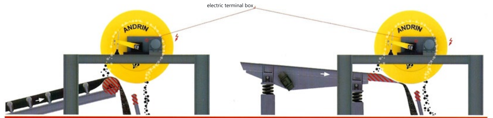
electromagnetic drums [Ø 320 - 1800 mm / width 400 - 3000 mm]
